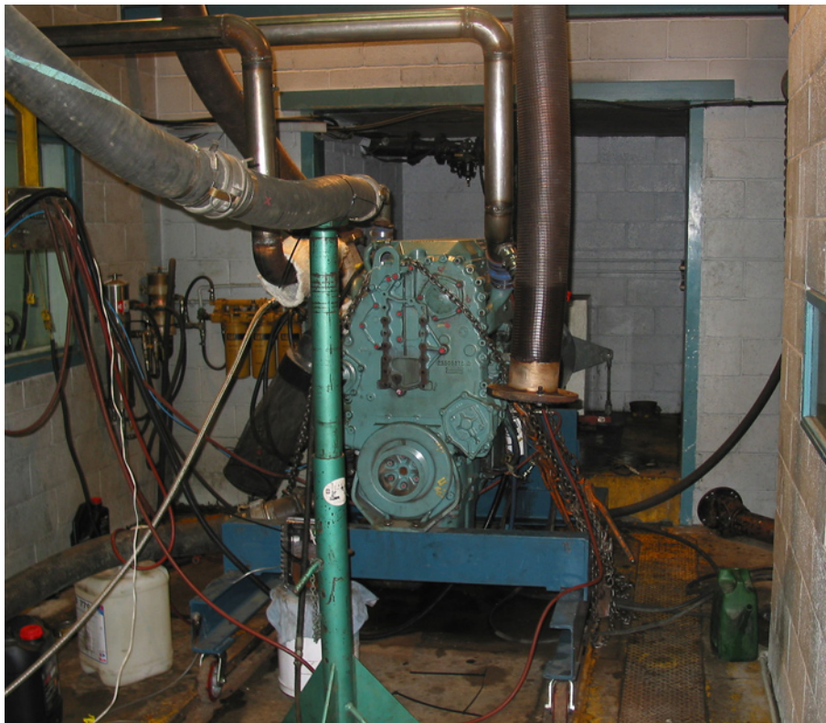
Detroit Series 60 DDEC III engine on test bed
